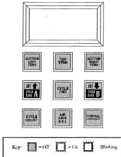
Figure 4-1 DES-42 C4 Control Panel with Buttons Off
